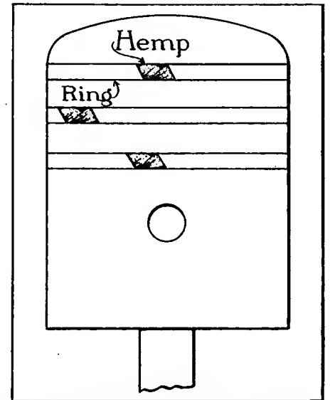
Fig. 4—Showing the appearance of the piston after the hemp is inserted
